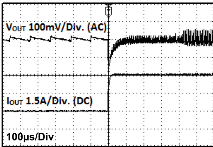
Fig 21: Load Response Characteristics (VIN=5V, VOUT=3.3V, IOUT=0 → 3A, FREQ=H, MODE=L)
