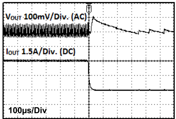
Fig 22: Load Response Characteristics (VIN=5V, VOUT=3.3V, IOUT=3A → 0, FREQ=H, MODE=L)
