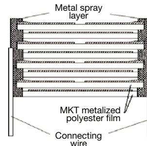
F1772-2 Extended metalized film with internal series connection design
