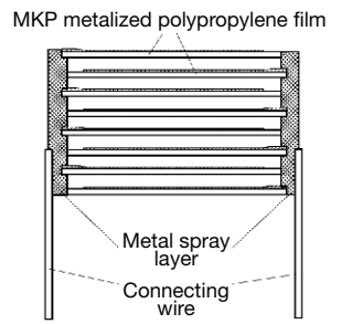
MKP1848 Extended Metalized Film Design
