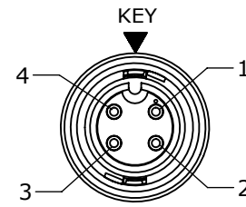
FACE VIEW P/N: CARA62804PXXX90
