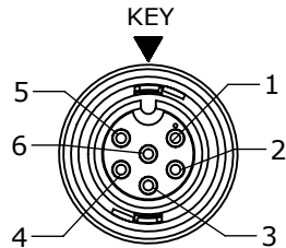
FACE VIEW P/N: CARA62806PXXX90
