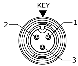
FACE VIEW P/N: CARA62803PXXX90
