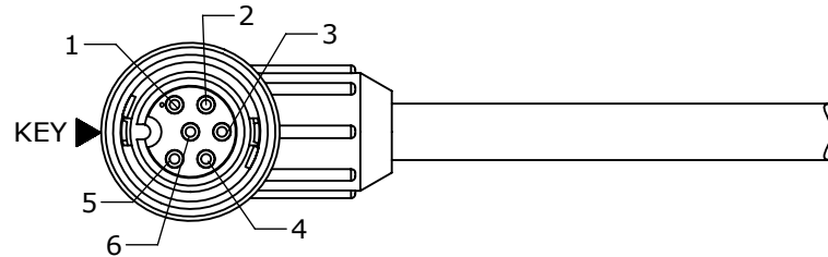
END "A" FACE VIEW SHOWN CARA62806PXXX90
