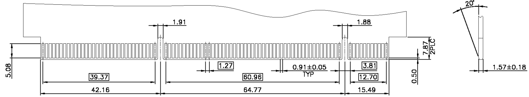
RECOMMENDED MATING PCB LAYOUT TOLERANCE: ±0.05mm
