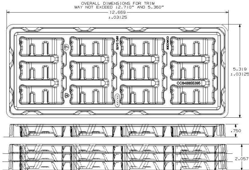
Figure 28. Through Hole Packaging Tray
